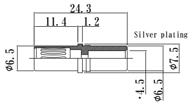
Crimp size : AWG#8, 10 JMD-TK-104 (Y)
