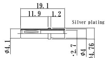
Crimp size : AWG#12, 14 JMD-TK-103 (Y)
