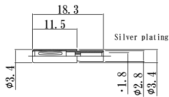
Crimp size : AWG#16 JMD52-04-05 (Y)
