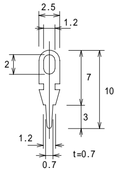
Metal Stamping
